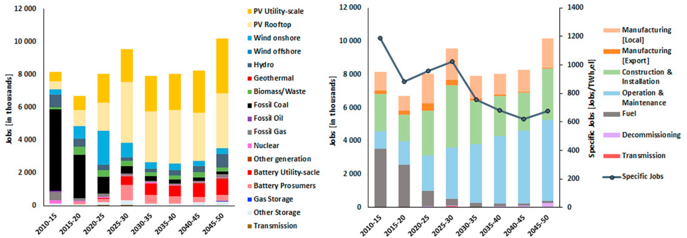
Fig. 8. Jobs created by the various power generation and storage technologies (left) and jobs created based on different categories with the development of electricity demand specific jobs (right) during the energy transition from 2015 to 2050 in Northeast Asia.
