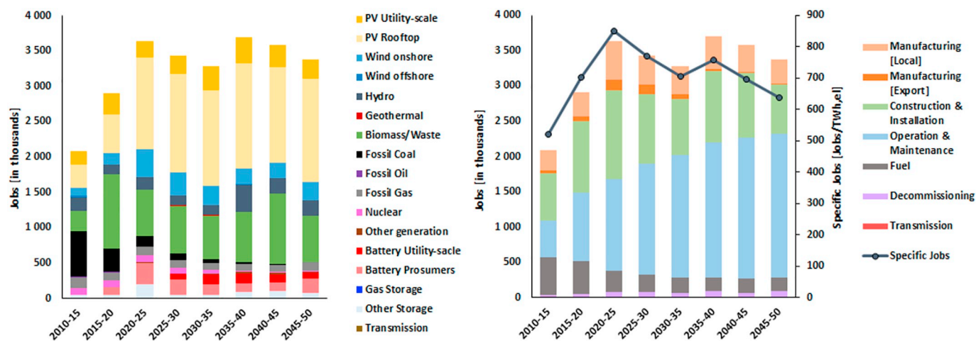
Fig. 3. Jobs created by the various power generation and storage technologies (left) and jobs created based on different categories with the development of electricity demand specific jobs (right) during the energy transition from 2015 to 2050 in Europe.
