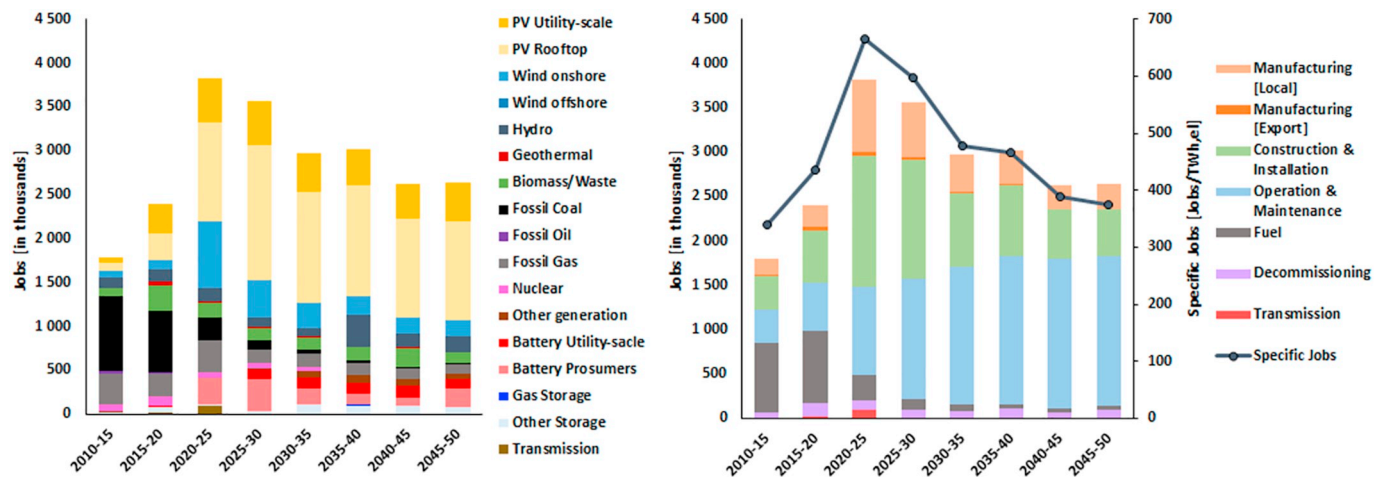
Fig. 10. Jobs created by the various power generation and storage technologies (left) and jobs created based on different categories with the development of electricity demand specific jobs (right) during the energy transition from 2015 to 2050 in North America.
