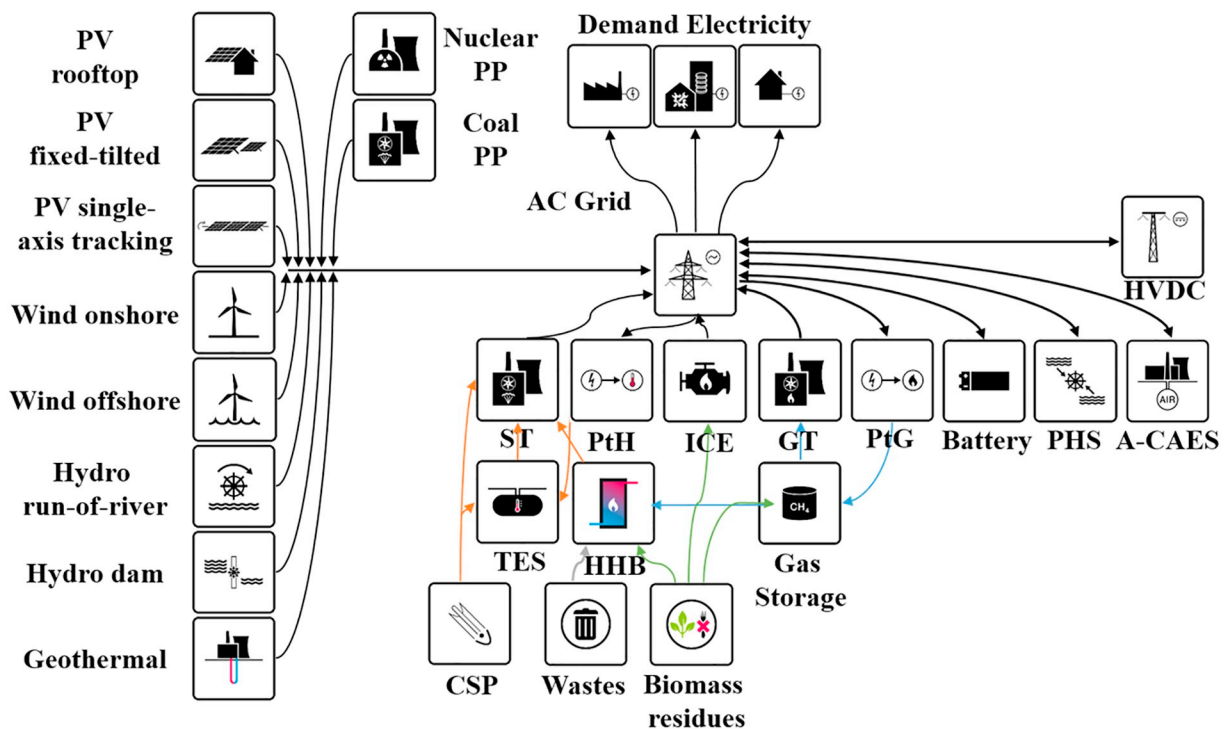
Fig. 2. The schematic representation of the LUT Energy System Transition model for the power sector with the various sources of power generation, transmission options, storage technologies and power demand sectors (Ram et al., 2017a).
