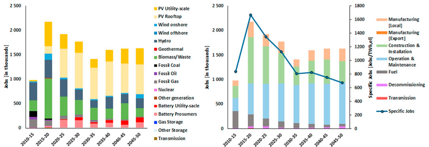
Fig. 11. Jobs created by the various power generation and storage technologies (left) and jobs created based on different categories with the development of electricity demand specific jobs (right) during the energy transition from 2015 to 2050 in South America.
