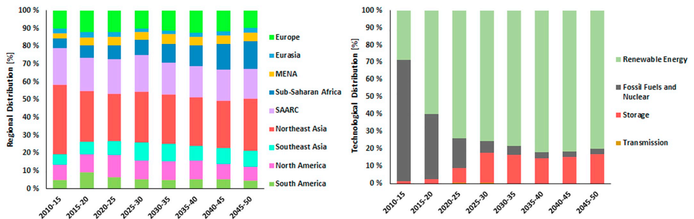
Fig. 13. Regional distribution of jobs created (left) and technological distribution of jobs created (right) during the energy transition from 2015 to 2050 globally.
