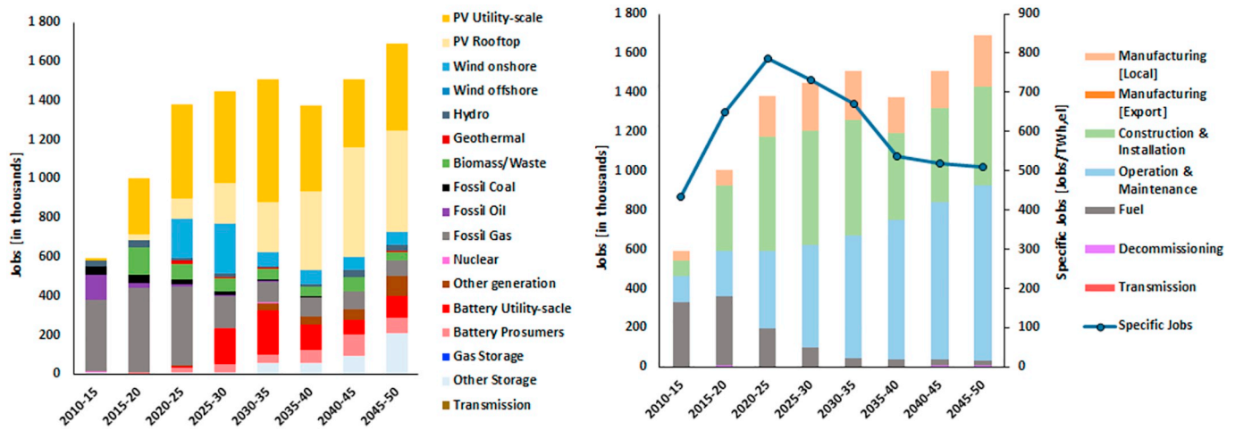
Fig. 5. Jobs created by the various power generation and storage technologies (left) and jobs created based on different categories with the development of electricity demand specific jobs (right) during the energy transition from 2015 to 2050 in the MENA region.
